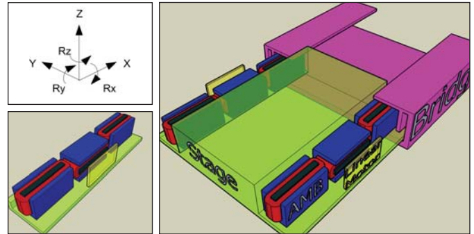
Figure 3. Basic design of AMB-Module (LEFT) and AMB High Precision Stage (RIGHT). The AMBs and the Linear Motor Coils are connected to the (green) moving part of the stage. The stationary (magenta) part of the stage serves as the counter material (bridge). This also contains magnets for the linear motor.
