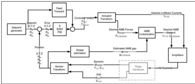
Figure 5. Basic control scheme: PID feedback and feed-forward with setpoint generator, geometric decoupling matrices and actuator linearization algorithm including air gap estimation.
