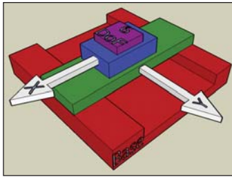
Figure 1. Standard High Precision Stage. The Y-module (green) and the X-module (blue) form the long stroke X-Y stage. The top (magenta) module is a 6 DoF short stroke module. This article describes the integration of the 6-DoF module with the X-module.
