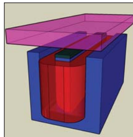
Figure 2. Basic design of Active Magnetic Bearing: E-core (blue), coil (red), magnet (black) and counter material (magenta).
