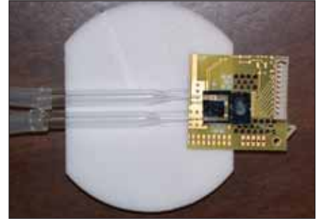
Prototype microchip device combining NIST's miniature atomic magnetometer with a fluid channel for studies of tiny samples. (Photo courtesy of NIST)
